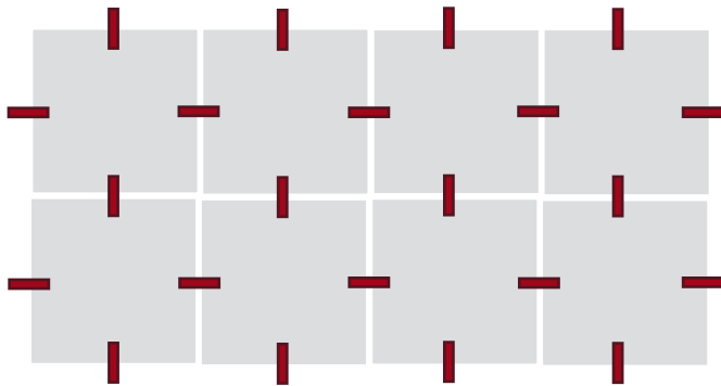
Regular clip layout for square tile. Example of 12" x 24" tile using 98 clips for 100 sq.ft.
